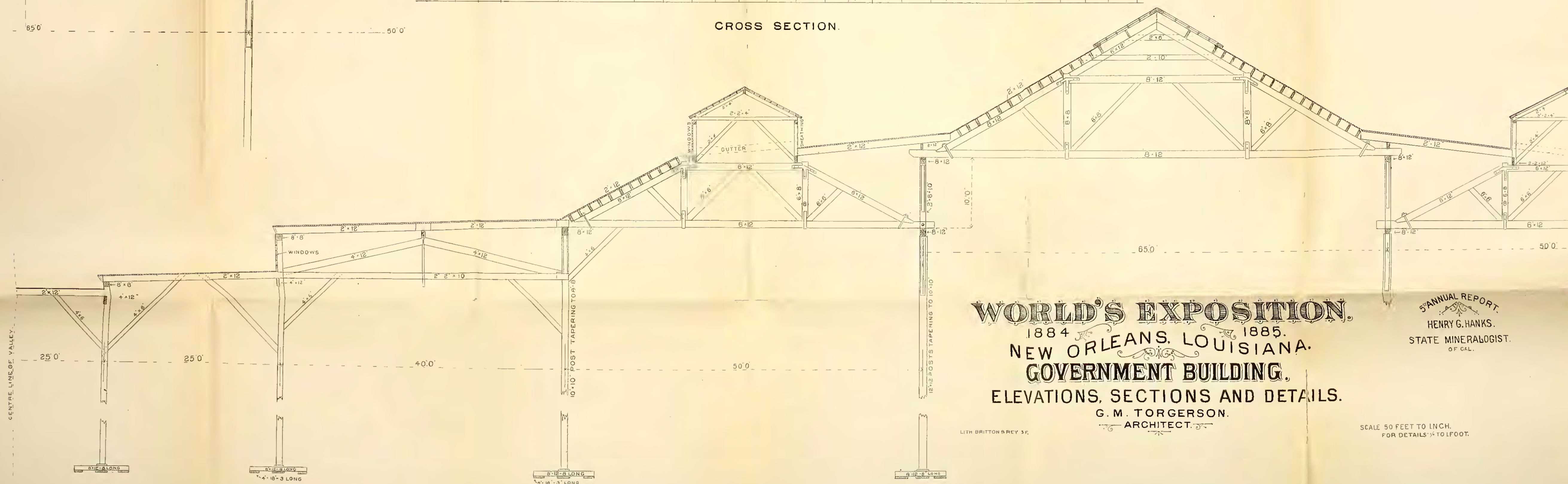
TRUSS IN CENTRE OF BUILDING
