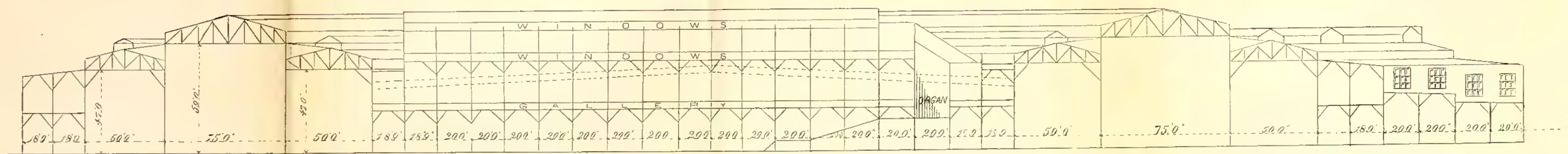
CROSS SECTION. DOTTED LINES INDICATE THE ROOFS OF THE VALLEYS
