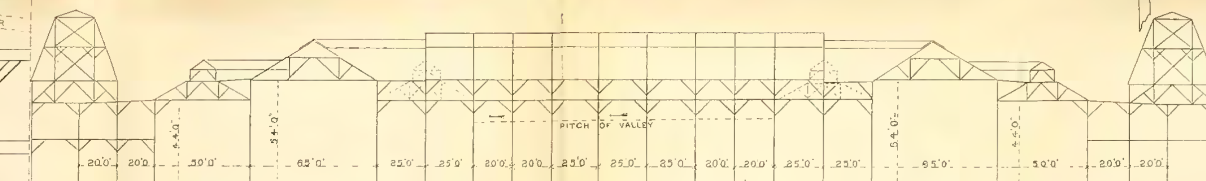
CROSS SECTION.
